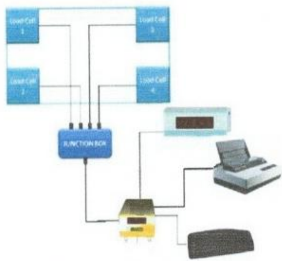
WEIGHBRIDGE GENERAL ARRANGEMENT
